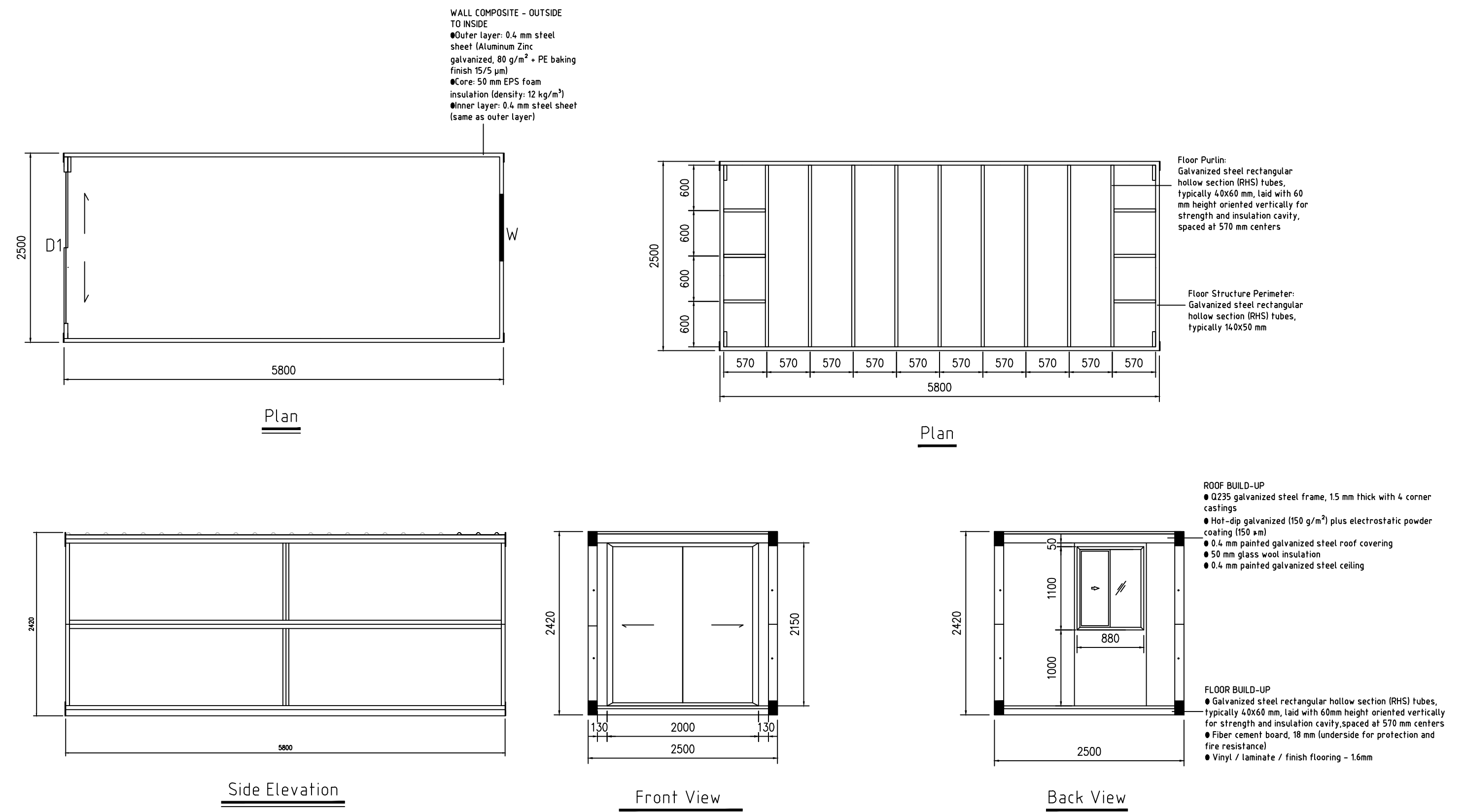
20ft foldable container with glass sliding door
