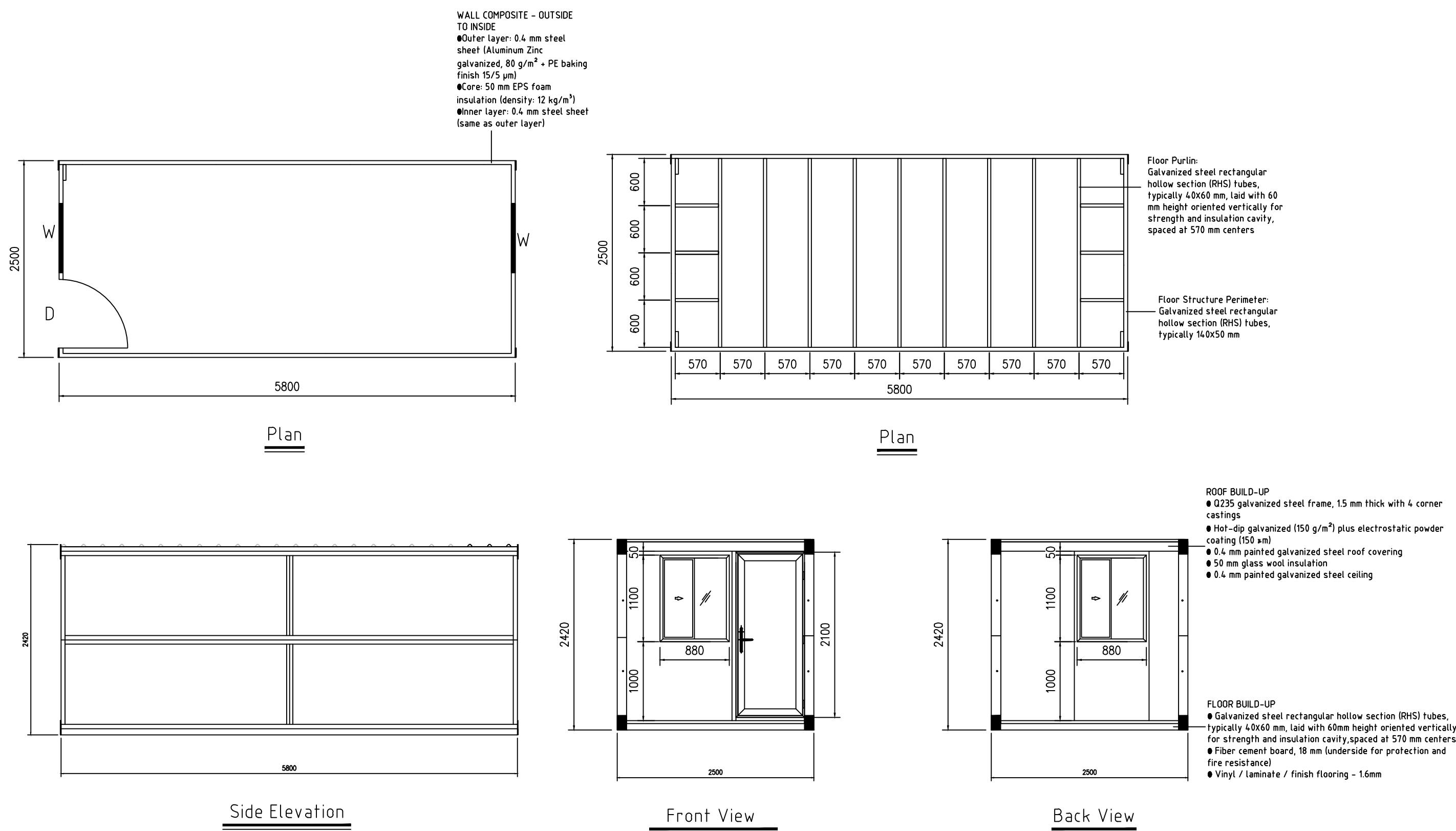
20ft foldable container with steel door
