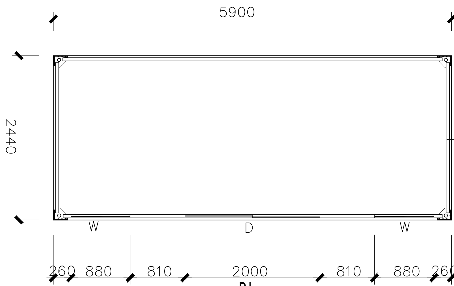
Plan
