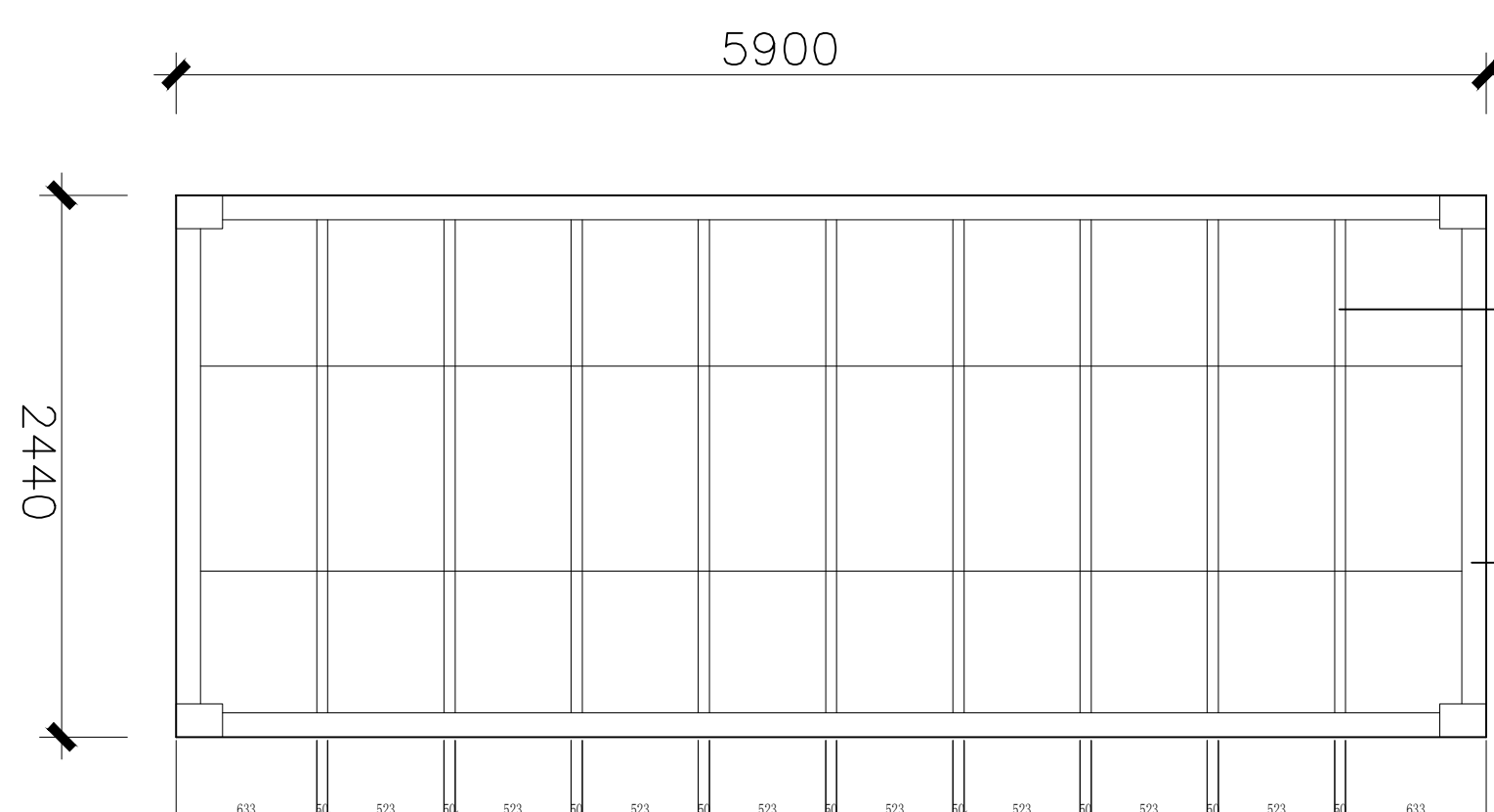
Floor
